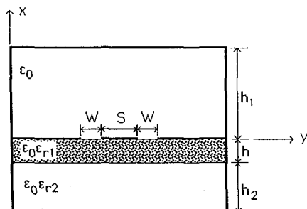
Figure 1: A cross section of a CPW inside a cavity.
