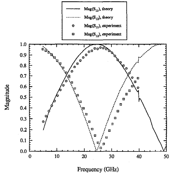
Figure 5: Scattering parameters of the straight open-end stub with air-bridges with L = 1100\mu m .
